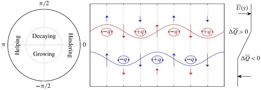
FIGURE 1. (Colour online) A pictorial representation of the wave interaction mechanism for the case of two Rossby waves. Here, q \sim -\Delta\bar{Q}\eta , where q is vorticity, \eta is displacement, and \Delta\bar{Q} is the magnitude of the vorticity jump of the background flow profile. Taking into account the sign of \Delta\bar{Q} at each jump, the q anomalies resulting from the \eta distribution are labelled accordingly. The top wave has a self-induced propagation to the left relative to the mean flow, and vice versa for the bottom wave, and both waves propagate counter to the mean flow. The waves interact with each other via the non-local velocity field induced by local vorticity anomalies, and the induced velocities decay with distance from vorticity anomalies, represented here by the length of the arrows. The waves may be held steady owing to counter-propagation relative to the mean flow, together with the mutual interaction between the waves, resulting in a phase-locked configuration. The waves can then constructively interfere and lead to instability. A phase difference regime diagram is given on the left, where the phase difference is defined as \Delta\epsilon = \epsilon_2 - \epsilon_1 , the lower wave displacement relative to the upper wave; the configuration here has \Delta\epsilon = -\pi/2 .
