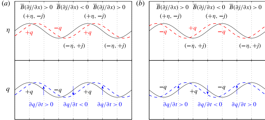
FIGURE 3. (Colour online) Pictorial representation for wave dynamics associated with \bar{B}(\partial j/\partial x) , with \bar{B} > 0 without loss of generality. The upper and lower panels are the \eta and q initial conditions, where (a) \eta \sim q and (b) \eta \sim -q . The solid black line shows tendencies associated with the chosen initial condition; grey dashed line (blue online; lower panels) is the influence of the \eta profile on q ; and grey dashed line (red online; upper panels) is the influence of the q profile on \eta . See text for description.
