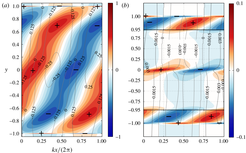
FIGURE 11. (Colour online) Representative eigenfunctions (normalised by the maximum absolute value of the vorticity) of the profile given in (5.1), both for k = 0.25 , but with (a) M = 0.8 and (b) M = 0.98 . The shading (red and blue online) is for positive and negative vorticity (respectively), and the displacement is plotted as labelled contours. In (b), the y scale is continuous between the panels (note the displacement contours are continuous in magnitude) but is not linear for display purposes.
