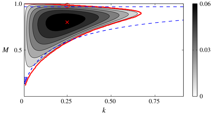
FIGURE 10. (Colour online) Growth rates (kc_i)_{full} of the full numerical solution associated with the basic state (5.1). Here, c_r = 0 for all unstable modes. The (red online) cross and circle correspond to the parameter location associated with the eigenfunction displayed in figure 11(a,b) respectively. The thick (red online) line is the stability boundary, and the dashed (blue online) curve is the resonance condition given in (5.3); numerical noise is present at small k partly due to the form of the phase speed c_A .
