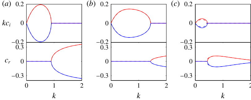
FIGURE 9. (Colour online) Line plots of the growth rate kc_i (upper row) and the phase speed c_r (lower row) associated with the growing and decaying solutions of the full solution (4.14), denoted by solid lines, and the \chi=0 solutions (4.17), denoted by dashed lines. These are evaluated at fixed M , with (a) M=0.5 , (b) M=0.75 and (c) M=0.9 . The \chi=0 solution is, for the most part, indistinguishable from the analytical solution.
