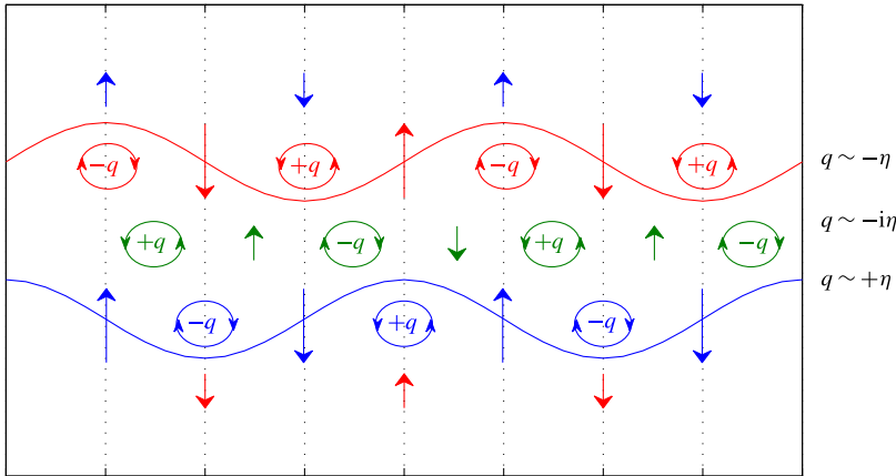
FIGURE 7. (Colour online) Schematic of how the critical layer contribution plays a role in the dynamics. Without the centre contribution (denoted online by the green parts), the dynamics of the two waves ( q \sim -\eta and q \sim +\eta ) are as in figure 1. The centre wave acts as a standing wave with q \sim -i\eta , with a resulting vorticity configuration as depicted in the figure. Then it is seen that the extra contributions act against the vorticity anomalies associated with the counter-propagating waves, and is thus a stabilising effect.
