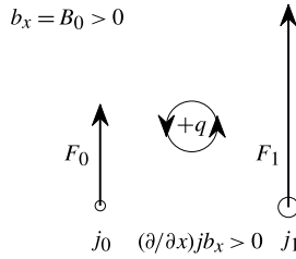
FIGURE 2. A pictorial representation of how the vorticity is generated by the Lorentz term \mathbf{j} \times \mathbf{B} = \nabla \cdot (\mathbf{j}\mathbf{B}) in two-dimensional incompressible MHD; see text for details.
