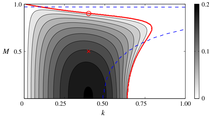
FIGURE 5. (Colour online) Growth rates (kc_i)_{full} of the full numerical solution associated with the basic state (4.5), with the thick (red online) curve denoting the stability boundary. Here, c_r = 0 for all unstable modes. The (red online) cross and circle correspond to the parameter location associated with the eigenfunction displayed in figure 6(a,b) respectively. The resonance condition is plotted as the dashed (blue online) line.
