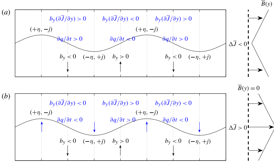
FIGURE 4. (Colour online) Pictorial representation for wave dynamics associated with b_y(\partial\bar{J}/\partial y) , the third term on the right-hand side of (2.5a), with (a) \bar{B}\Delta\bar{J} < 0 and (b) \bar{B}\Delta\bar{J} > 0 ; without loss of generality, \bar{B} > 0 . The initial conditions are given in black; and the resulting tendencies arising from the choice of initial conditions are given in grey (blue online). See text for more details.
