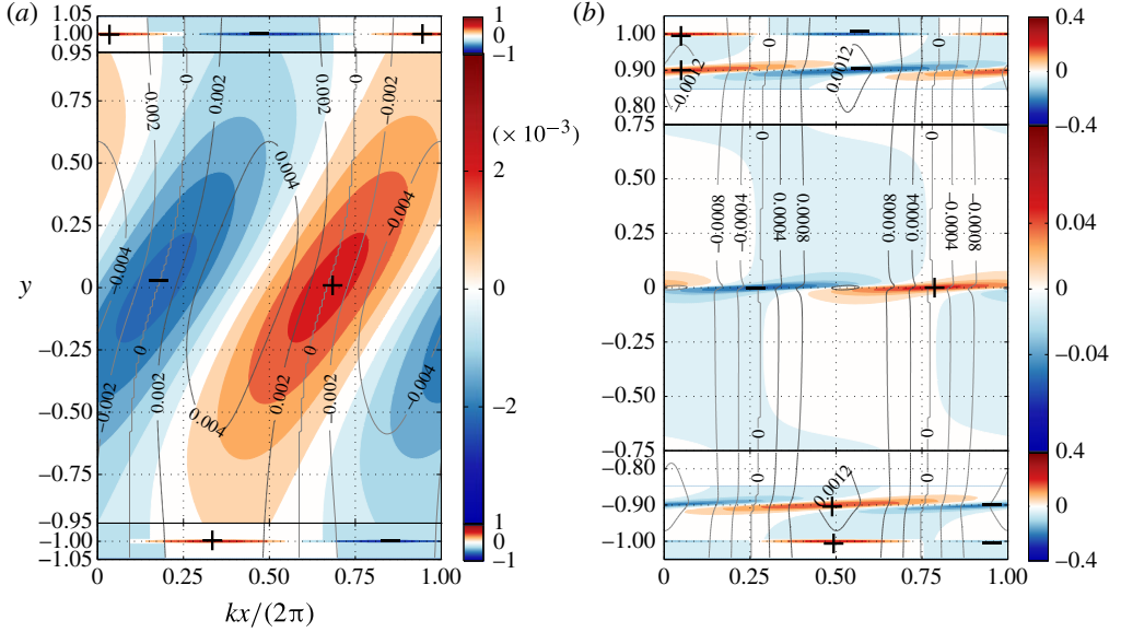
FIGURE 6. (Colour online) Representative eigenfunctions (normalised by the maximum absolute value of q ) of the profile given in (4.5), both for k=0.4 , but with (a) M=0.5 and (b) M=0.9 . The shading (red and blue online) is for positive and negative q (respectively), and \eta is plotted as labelled contours; note the difference in the colour scales used between the panels. The y scale is continuous between the panels (note the displacement contours are continuous in magnitude) but is not linear for display purposes.
