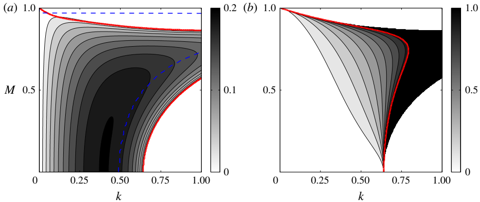
FIGURE 8. (Colour online) Results from taking only two interfaces, for the profile given in (4.5): (a) shows the growth rates (kc_i)_{int} of the approximated solution from (4.14); (b) shows the weighted error E = 1 - (kc_i)_{full}/(kc_i)_{int} . The thick (red online) line here is the stability boundary of the full solution in figure 5, while the resonance condition from (4.7) is shown as the dashed (blue online) curve.
